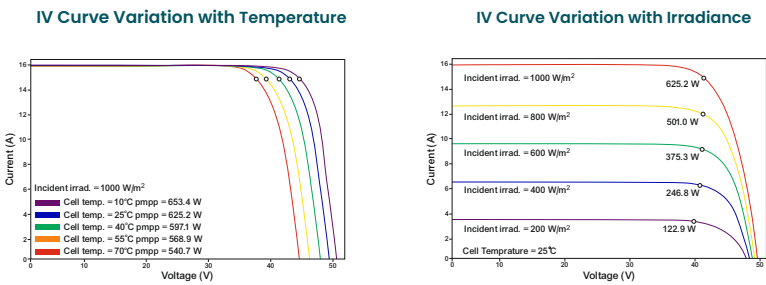
IV Curves for Front-Side Illumination of 625 Wp Panel
